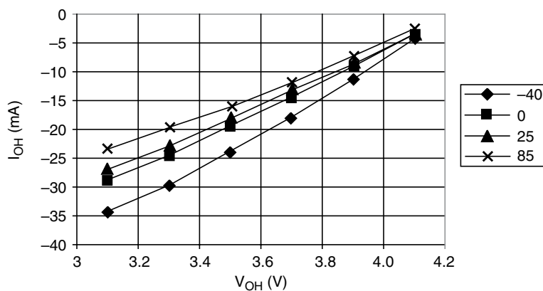
Figure 19-2. Typical High-Side Driver Characteristics – Port PTA7–PTA0 ( V_{DD} = 4.5 \text{ Vdc} )
