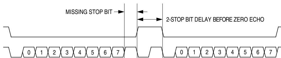
Figure 18-14. Break Transaction
