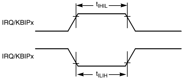
Figure 12. IRQ/KBIPx Timing
