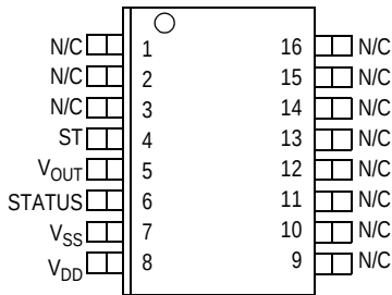
Figure 2. Pin Connections
