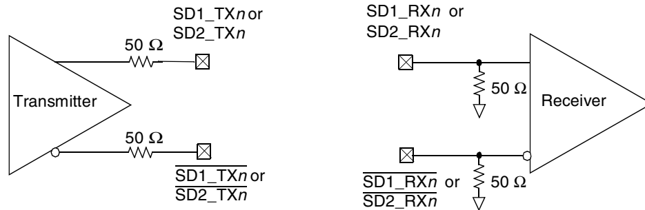
Figure 65. SerDes Transmitter and Receiver Reference Circuits
