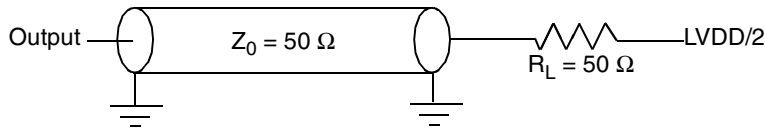
Figure 17. eTSEC AC Test Load
