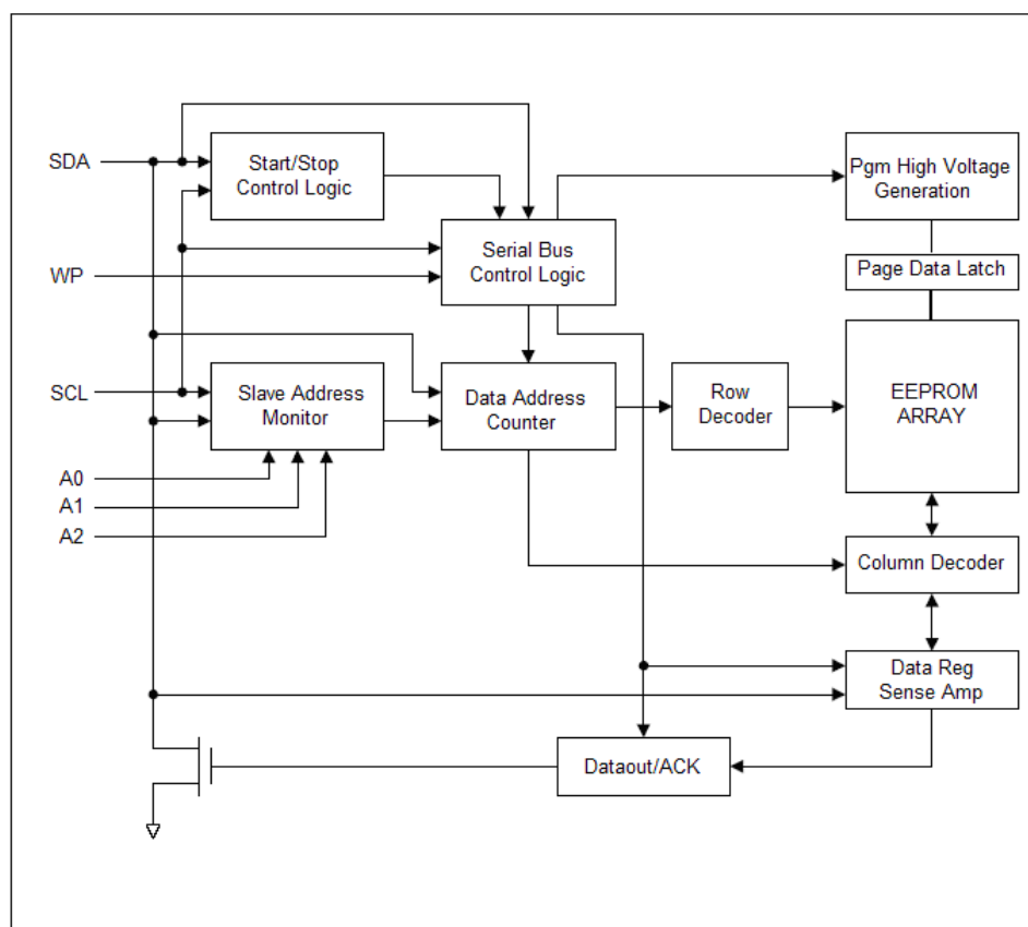
Figure 2: Block Diagram
