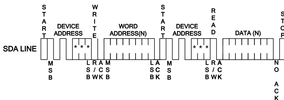
Figure 9: Random Read
