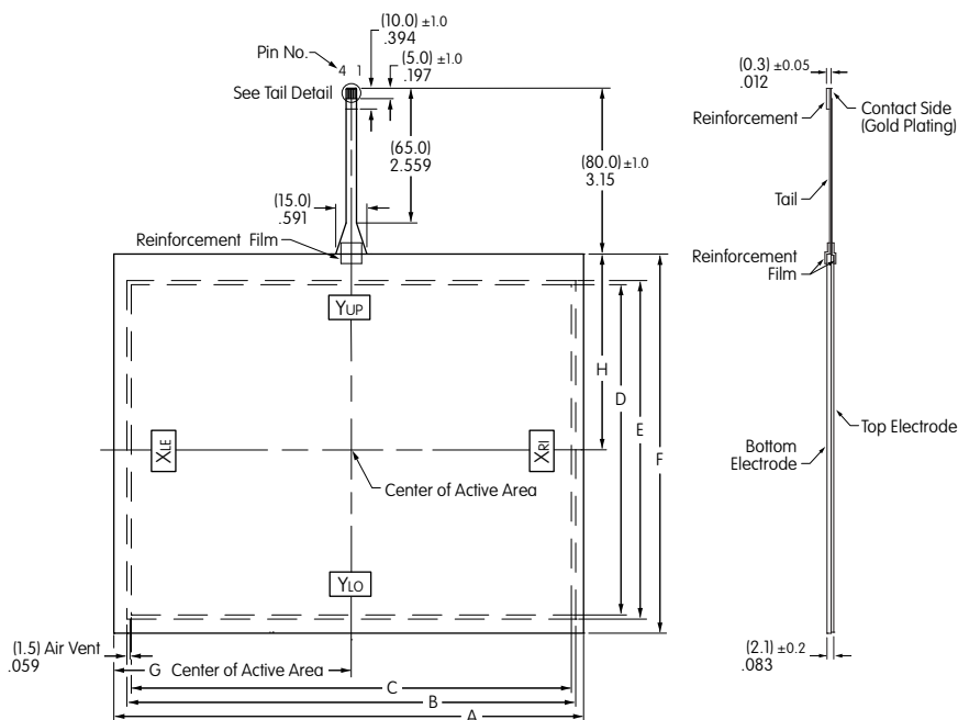
Typical Dimensions for Vertical Frame
