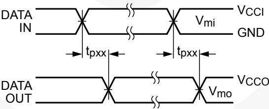
Figure 6. Waveform for Inverting and Non-Inverting Functions
