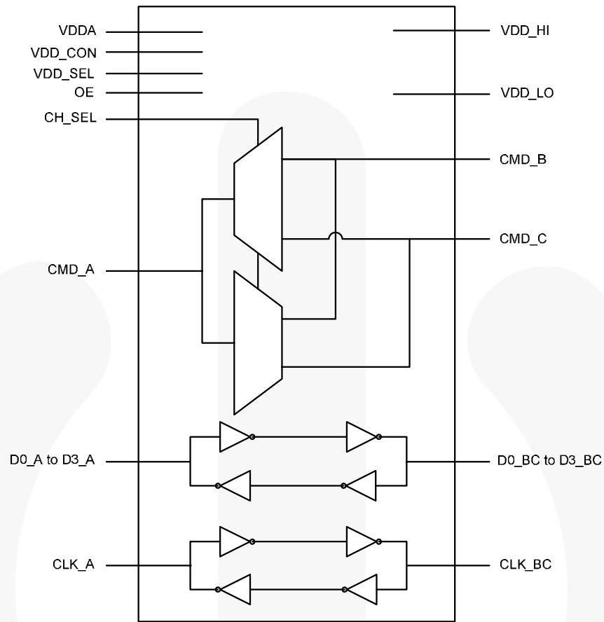
Figure 4. Function Diagram
