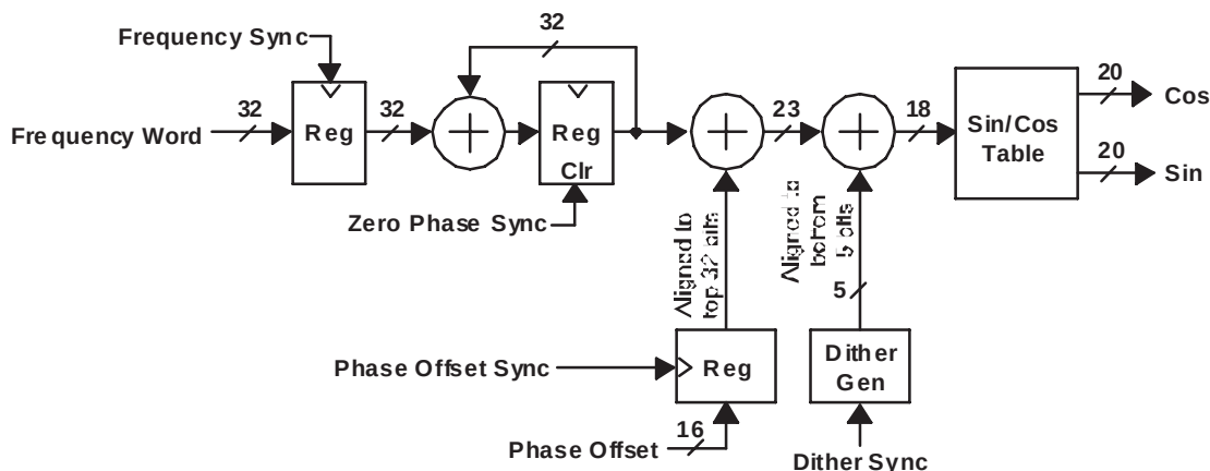
Figure 8. Receive Number Controlled Oscillator
