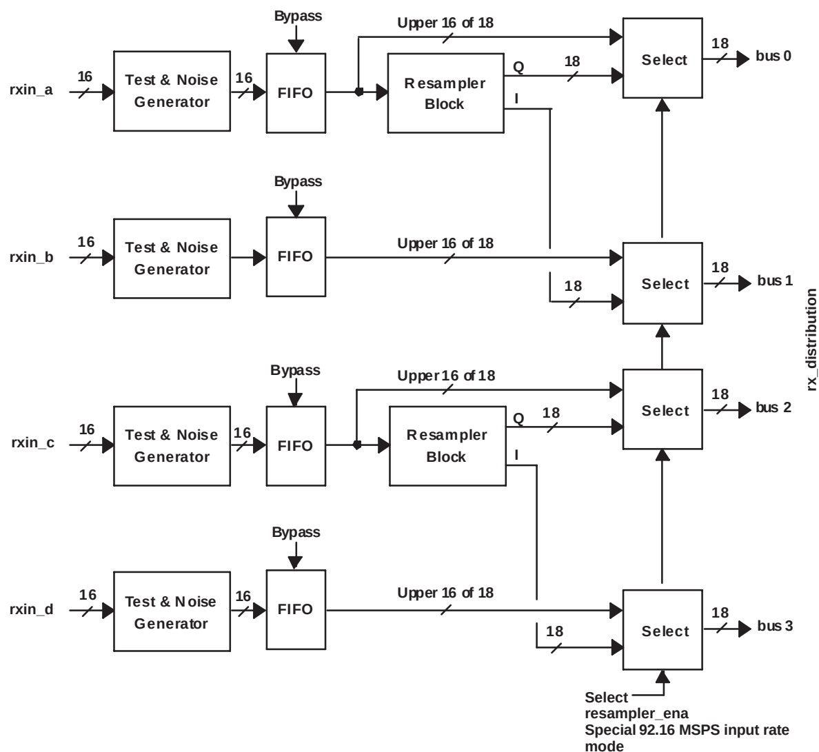
Figure 2. Receive Input Interface
