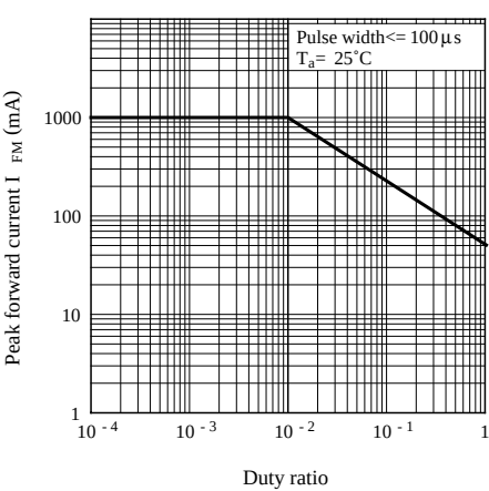
Fig. 2 Peak Forward Current vs. Duty Ratio
