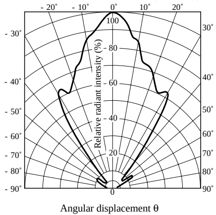
Fig. 9 Radiation Diagram (T a = 25°C)
