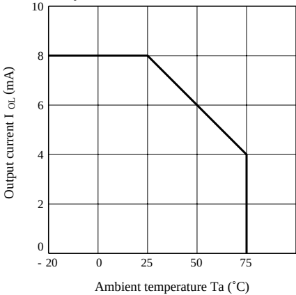
Fig. 1 Output Current vs. Ambient Temperature
