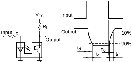
Test Circuit for Response Time
