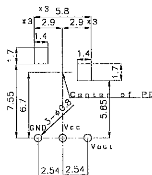
Example of mounting drawing from solder side(Reference)
