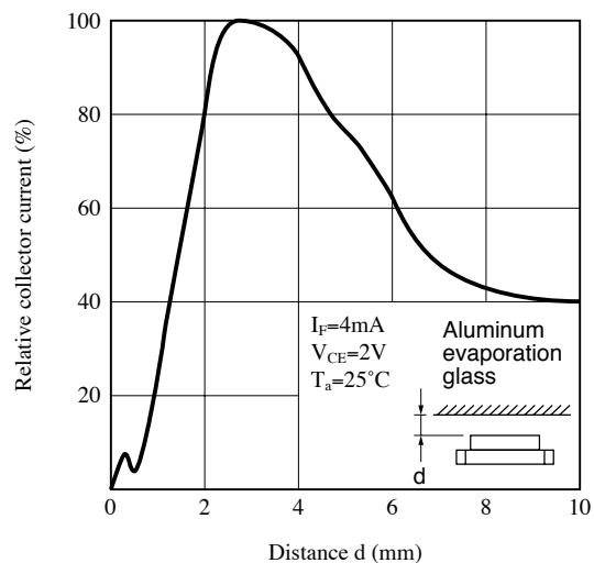
Fig.8 Relative Collector Current vs. Distance (Reference)
