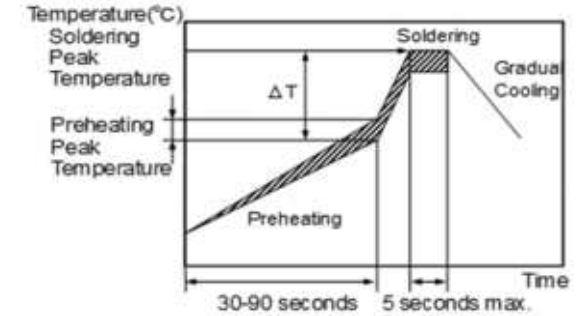
[ Allowable Flow Soldering Temperature and Time ]
