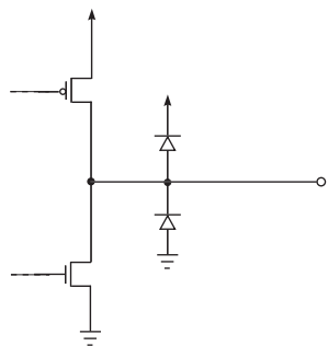
Figure 3-8: Indicator Outputs: SD/\overline{HD} , LD
