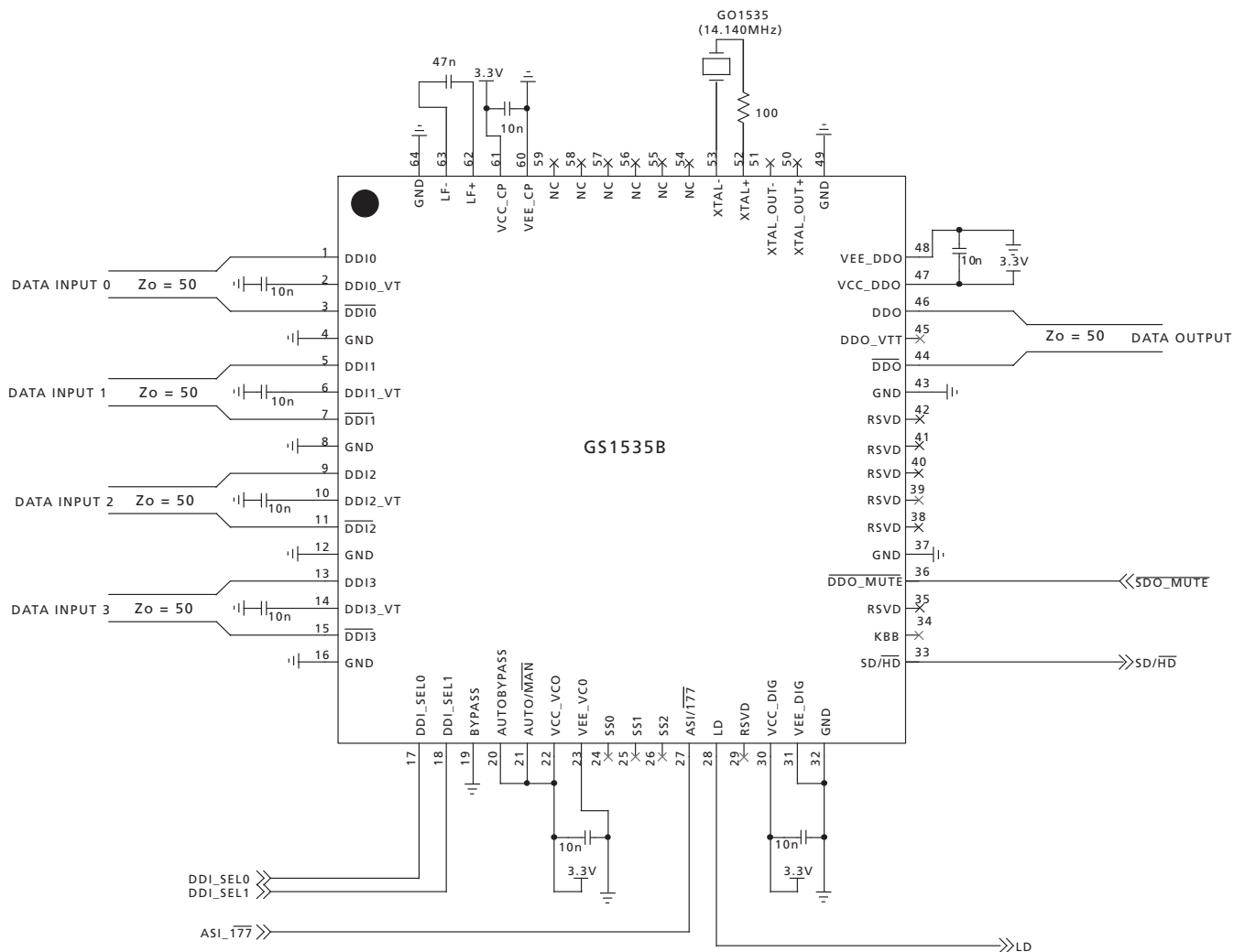
Figure 5-1: GS1535B Typical Application Circuit
