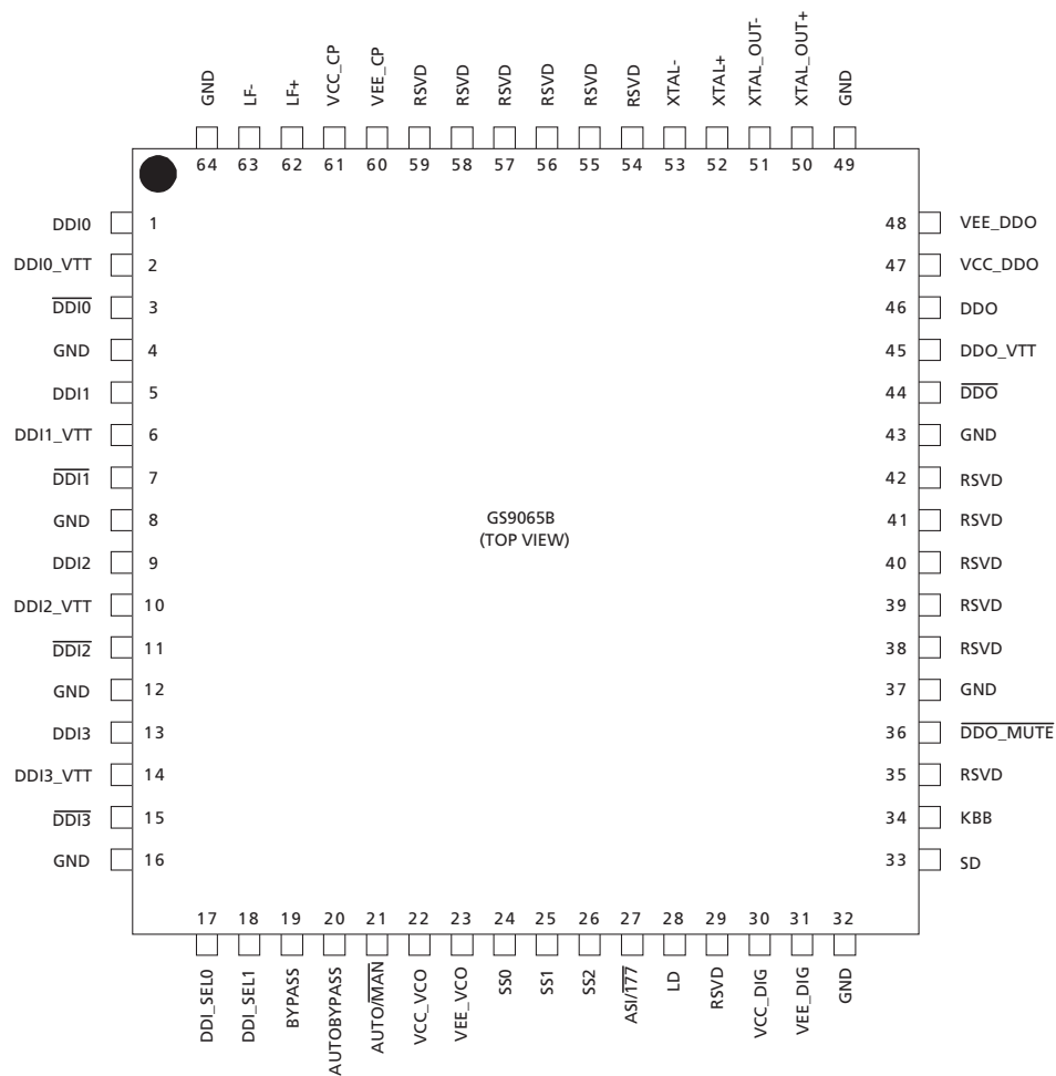
Figure 1-2: 64-Pin LQFP
