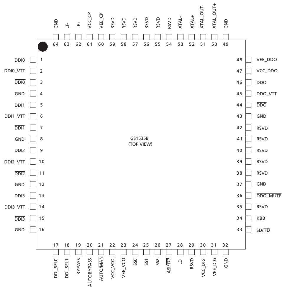
Figure 1-1: 64-Pin LQFP
