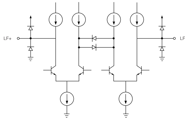
Figure 2-4: Loop Filter
