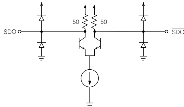
Figure 2-3: Serial Data Outputs
