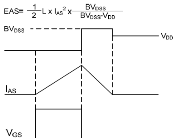
Figure 12. EAS Waveform
