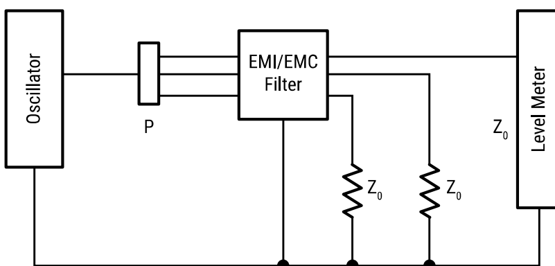
Measuring Circuit - Common Mode
