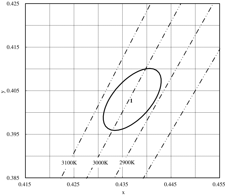
Chromaticity Diagram
