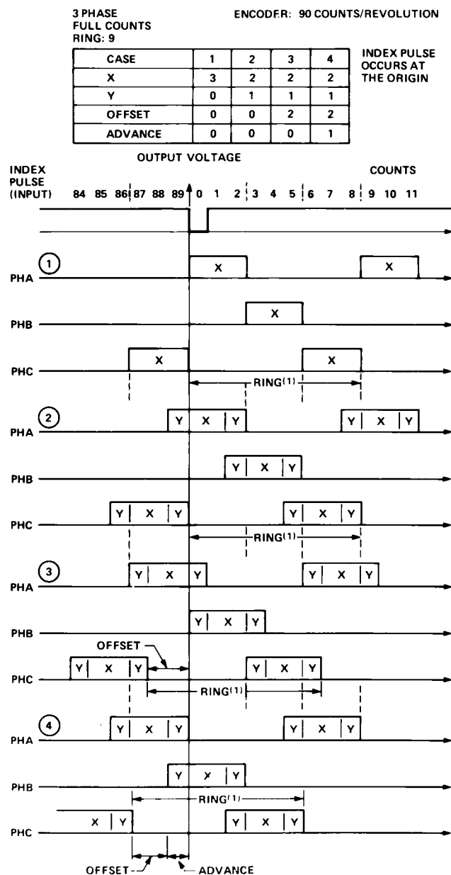
Figure 10. Commutator Configuration.
