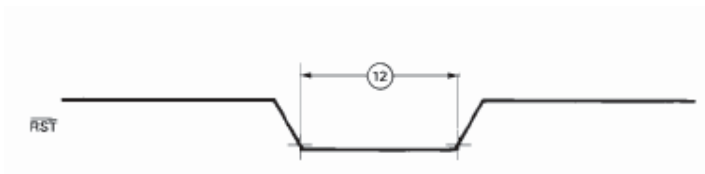
Figure 1. Reset Waveform
