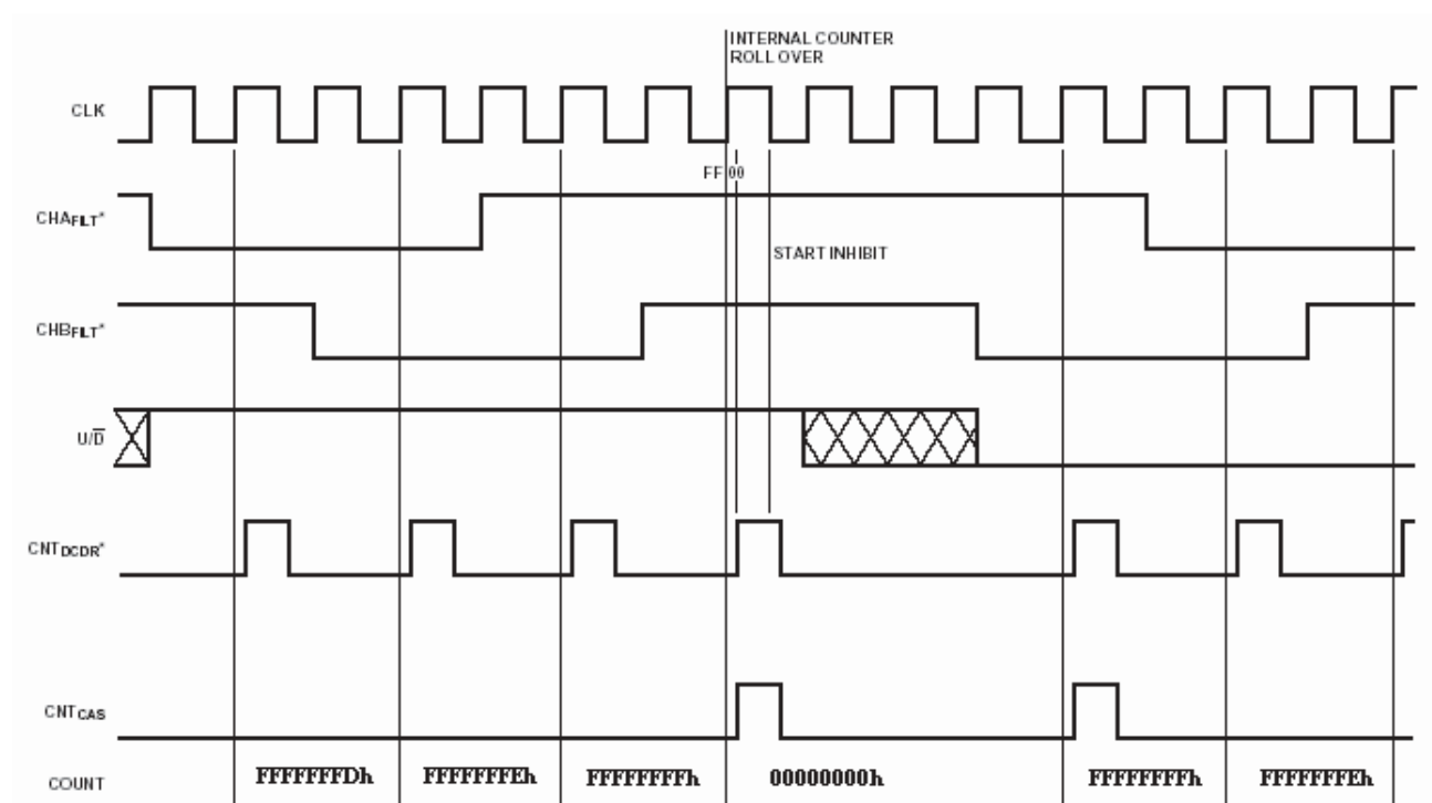
Figure 12. Decode and Cascade Output Diagram (4x)
