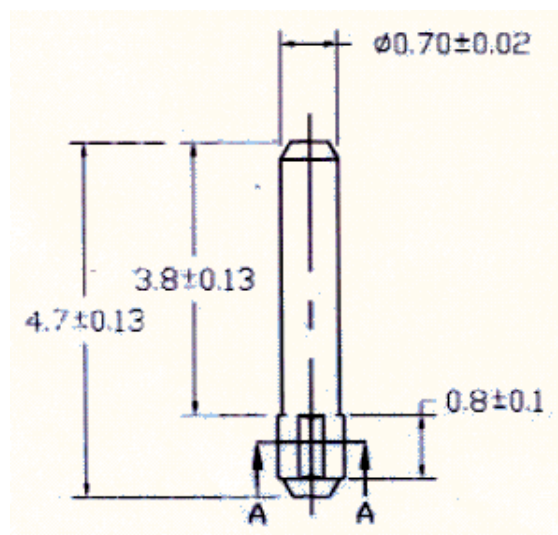
PIN DRAWING
