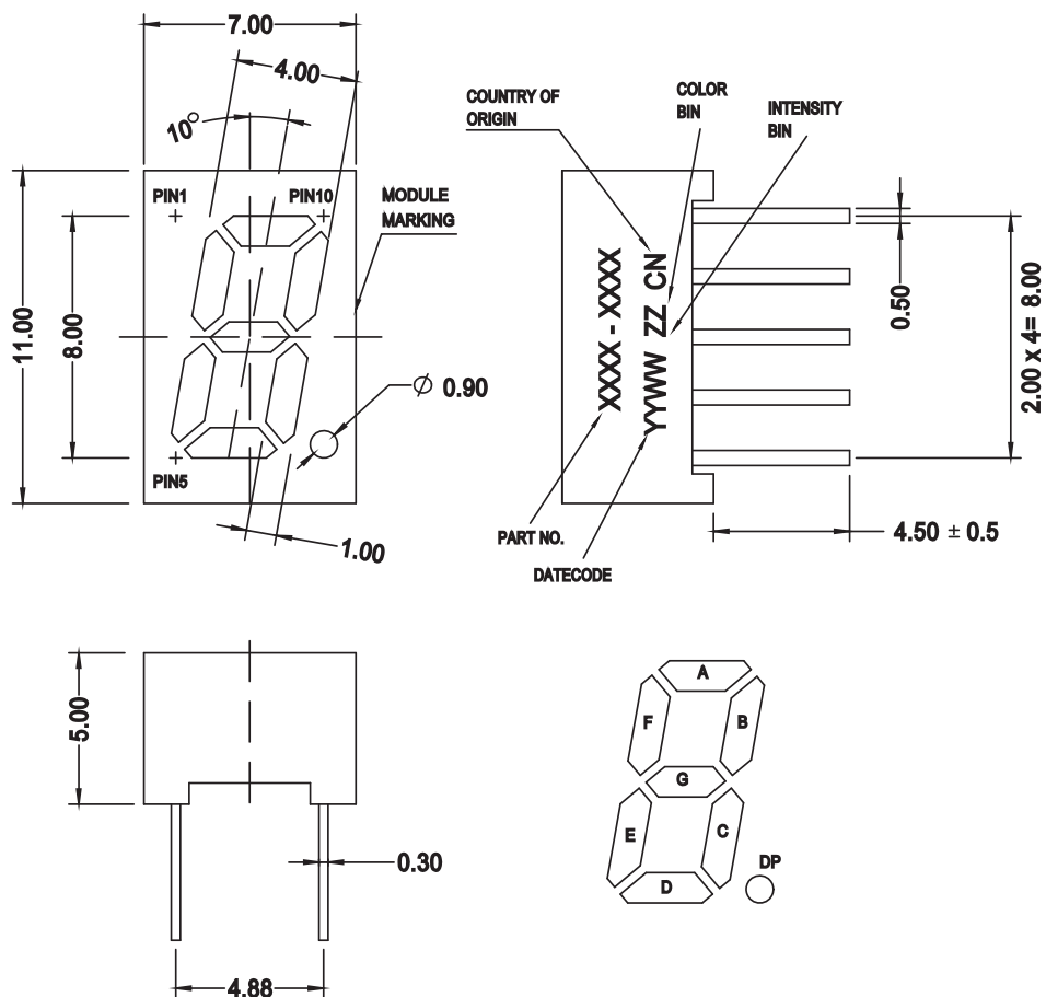
Figure 1: Package Drawing
