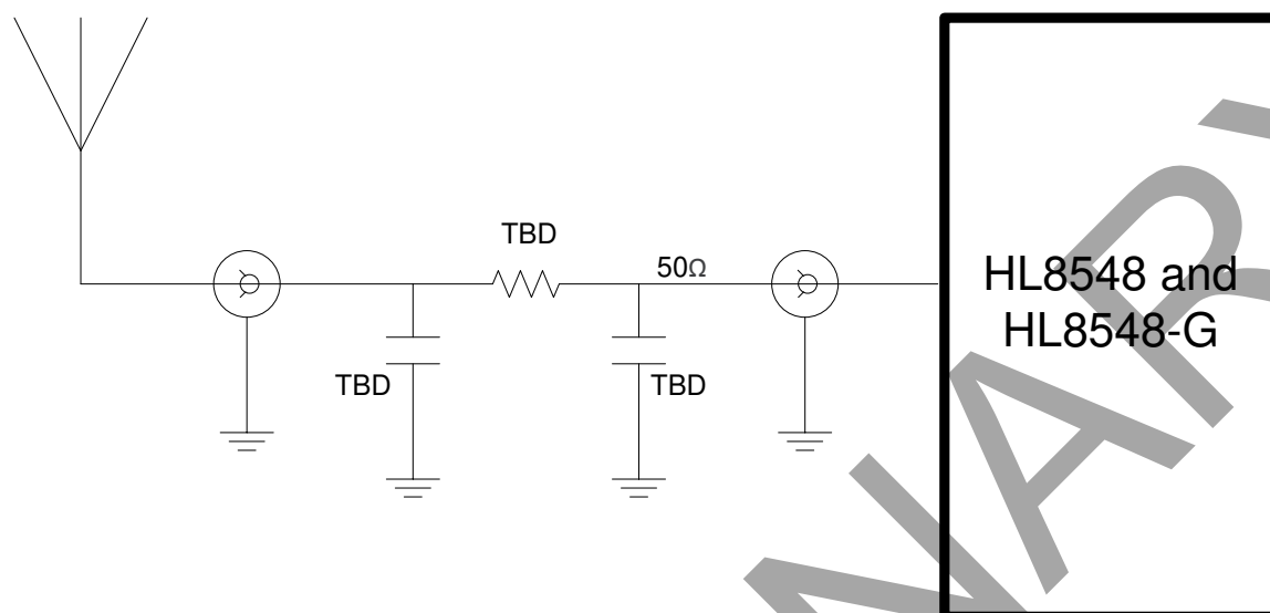
Figure 7. Antenna Connection
