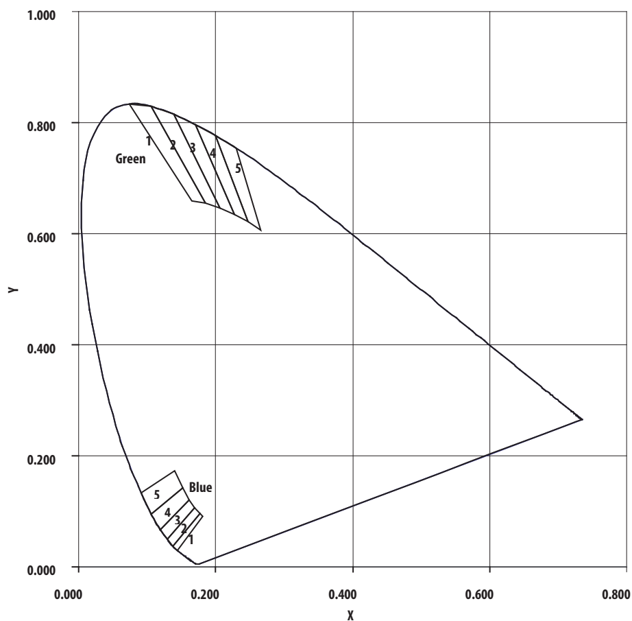
Avago Color Bin on CIE 1931 Chromaticity Diagram
