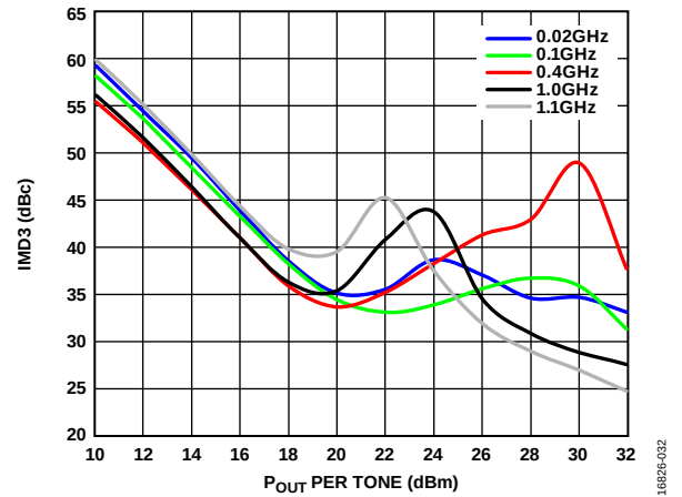
Figure 32. IMD3 vs. P_{OUT} per Tone, V_{DD} = 24\text{ V}
