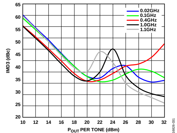
Figure 31. IMD3 vs. P_{OUT} per Tone, V_{DD} = 30\text{ V}
