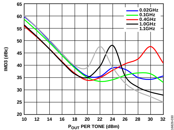
Figure 30. Output Third-Order Intermodulation (IMD3) vs. P_{OUT} per Tone, V_{DD} = 26\text{ V}
