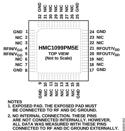
Figure 2. Pin Configuration
