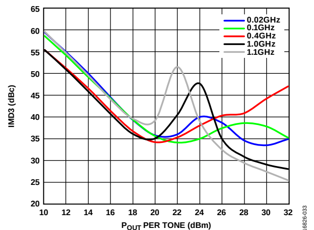
Figure 33. IMD3 vs. P_{OUT} per Tone, V_{DD} = 28\text{ V}
