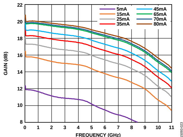
Figure 23. Gain vs. Frequency for Various Supply Currents ( I_{DD} ), V_{DD} = 5\text{ V}
