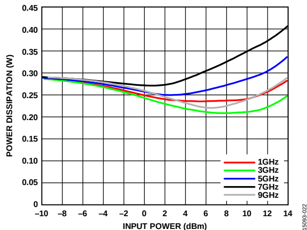
Figure 22. Power Dissipation vs. Input Power for Various Frequencies, T_A = 85^\circ\text{C}
