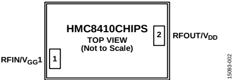
Figure 2. Pad Configuration
