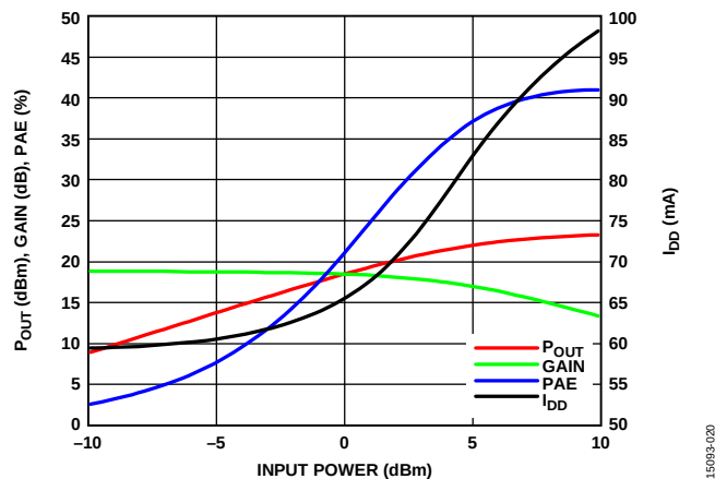
Figure 20. P_{OUT} , Gain, PAE, and Supply Current ( I_{DD} ) with RF Applied ( I_{DD} ) vs. Input Power at 5 GHz
