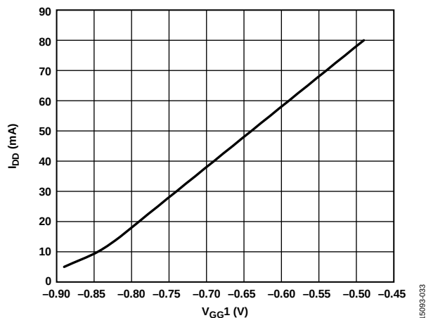
Figure 33. Supply Current ( I_{DD} ) vs. V_{GG1} , V_{DD} = 5 V, Representative of a Typical Device
