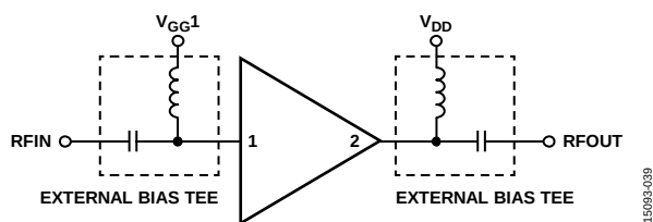
Figure 40. Application Circuit
