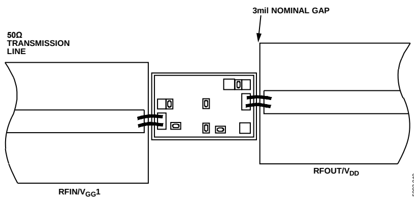
Figure 41. Assembly Diagram
