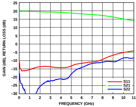
Figure 6. Gain and Return Loss vs. Frequency
