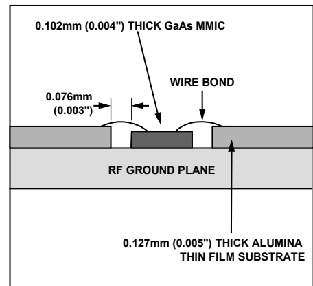
Figure 38. Die Without the Moly Tab
