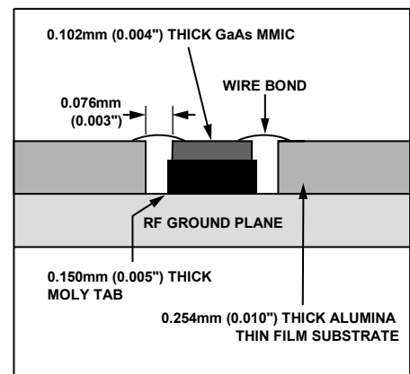
Figure 39. Die With the Moly Tab
