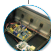
Mounting PCB on the GP bar and attaching electronic component to heatsink side frame
