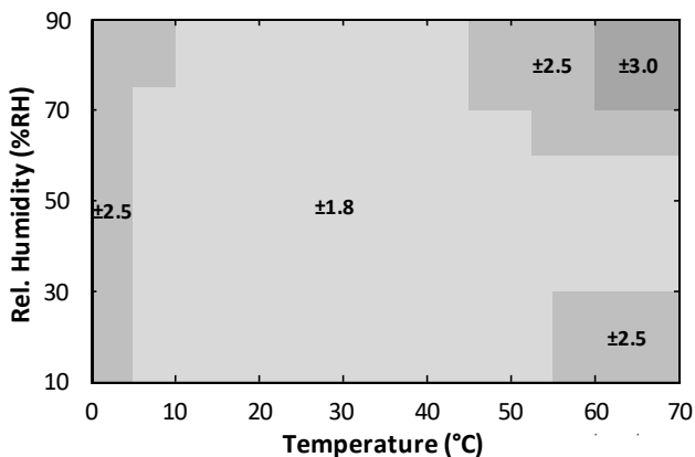
Figure 6. HS3002 RH Accuracy over Temperature
