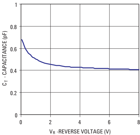
Figure 3. Total Capacitance vs. Reverse Bias
