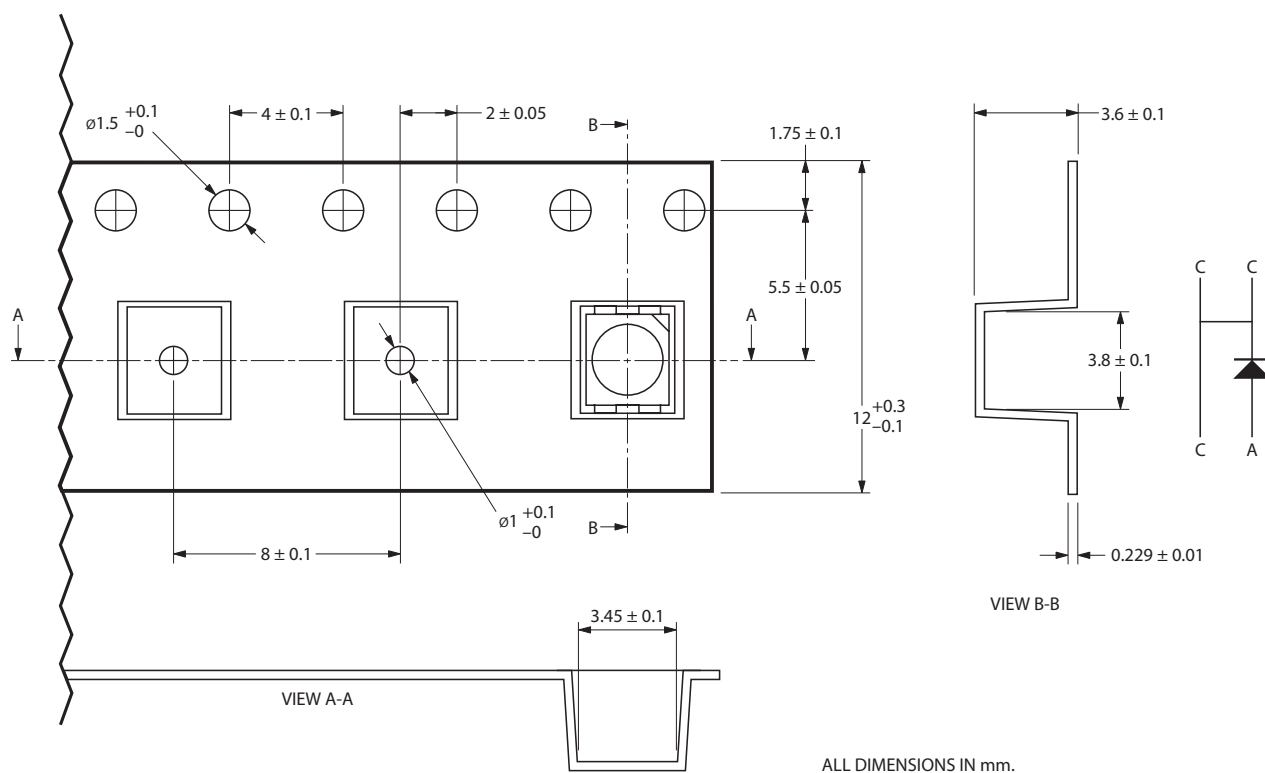
Figure 13. Tape dimensions
