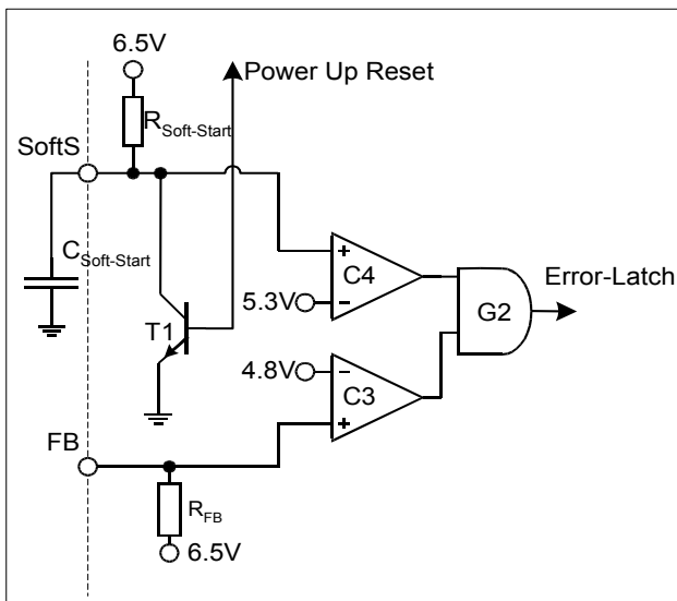
Figure 20 FB-Detection
