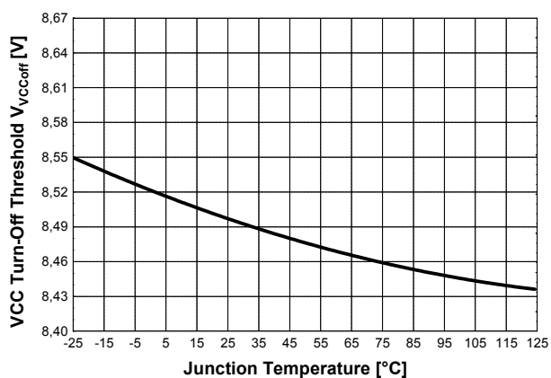
Figure 27 VCC Turn-Off Threshold V_{VCCoff} vs. T_j
