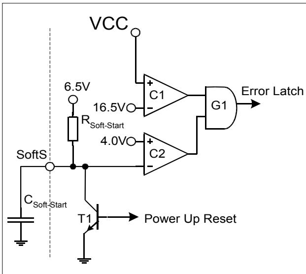
Figure 22 Overvoltage Detection
