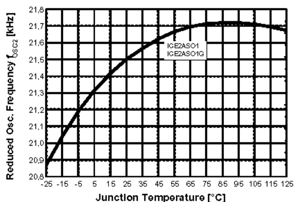
Figure 32 Reduced Osc. Frequency f_{OSC2} vs. T_j
