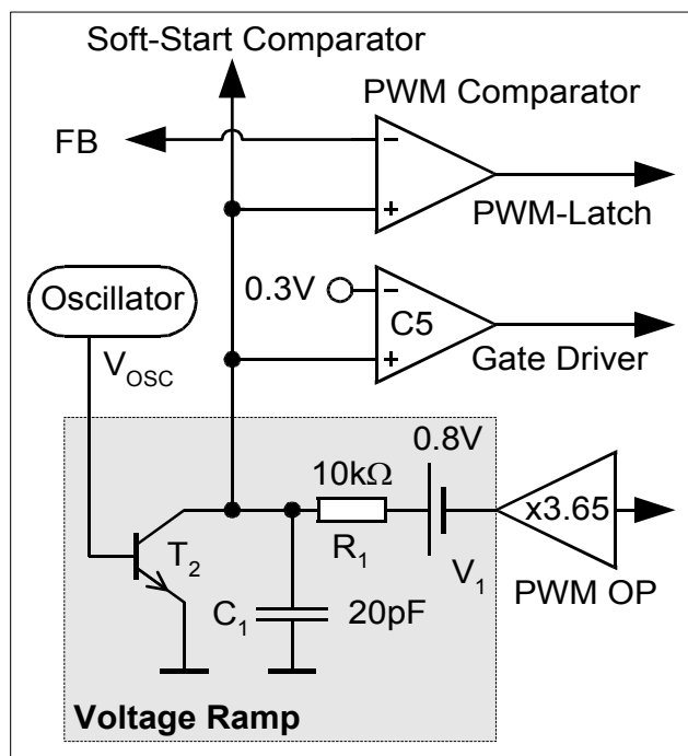
Figure 6 Improved Current Mode
