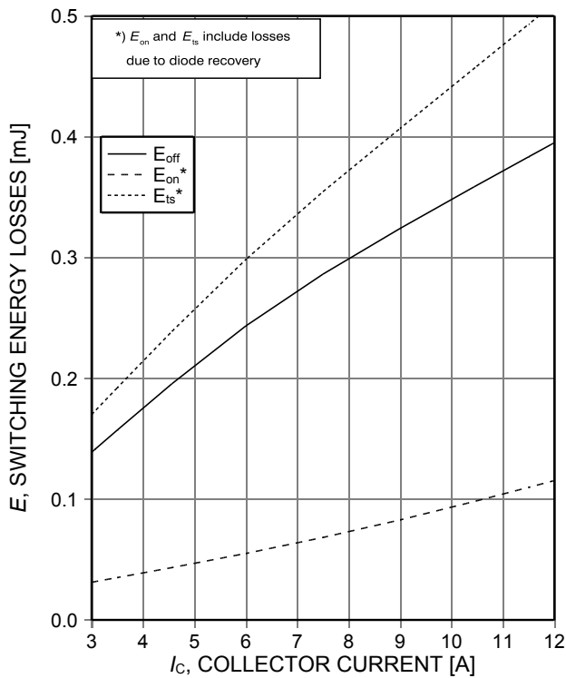
Figure 13. Typical switching energy losses as a function of collector current (inductive load, T_{vj}=175^\circ\text{C} , V_{CE}=400\text{V} , V_{GE}=15/0\text{V} , r_G=14.7\Omega , Dynamic test circuit in Figure E. Used diode: SDP04S60)
