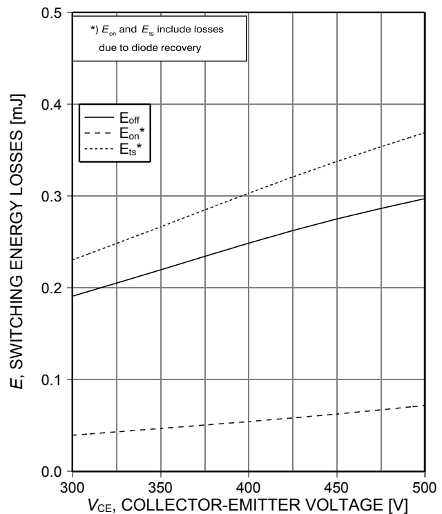
Figure 16. Typical switching energy losses as a function of collector emitter voltage (inductive load, T_{vj}=175^\circ\text{C} , V_{GE}=15/0\text{V} , I_C=6\text{A} , r_G=14.7\Omega , Dynamic test circuit in Figure E. Used diode: SDP04S60)
