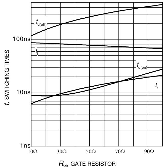
Figure 10. Typical switching times as a function of gate resistor (inductive load, T_J = 175^\circ\text{C} , V_{CE} = 400\text{V} , V_{GE} = 0/15\text{V} , I_C = 6\text{A} , Dynamic test circuit in Figure E)
