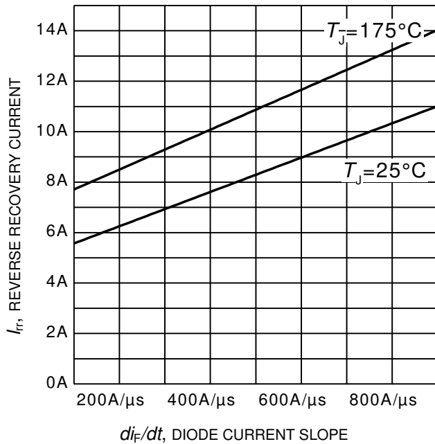
Figure 25. Typical reverse recovery current as a function of diode current slope
