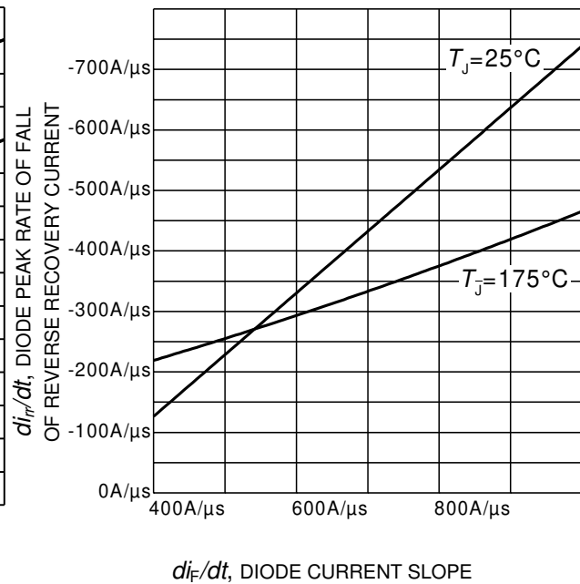
Figure 26. Typical diode peak rate of fall of reverse recovery current as a function of diode current slope
