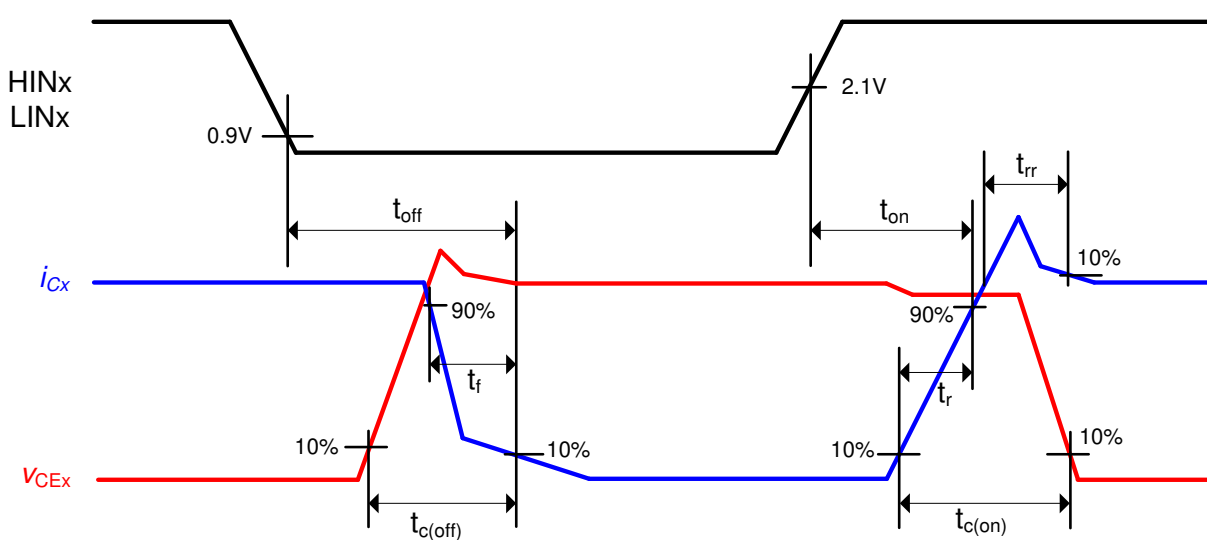
Figure 8 Switching times definition
