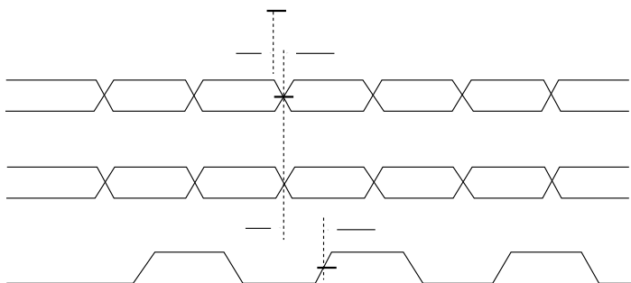
Figure 49. RGMII Receive Signal Timing Diagram Original
