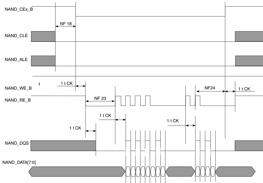
Figure 35. Samsung Toggle Mode Data Read Timing
