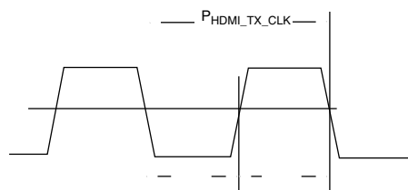
Figure 54. TMDS Clock Signal Definitions
