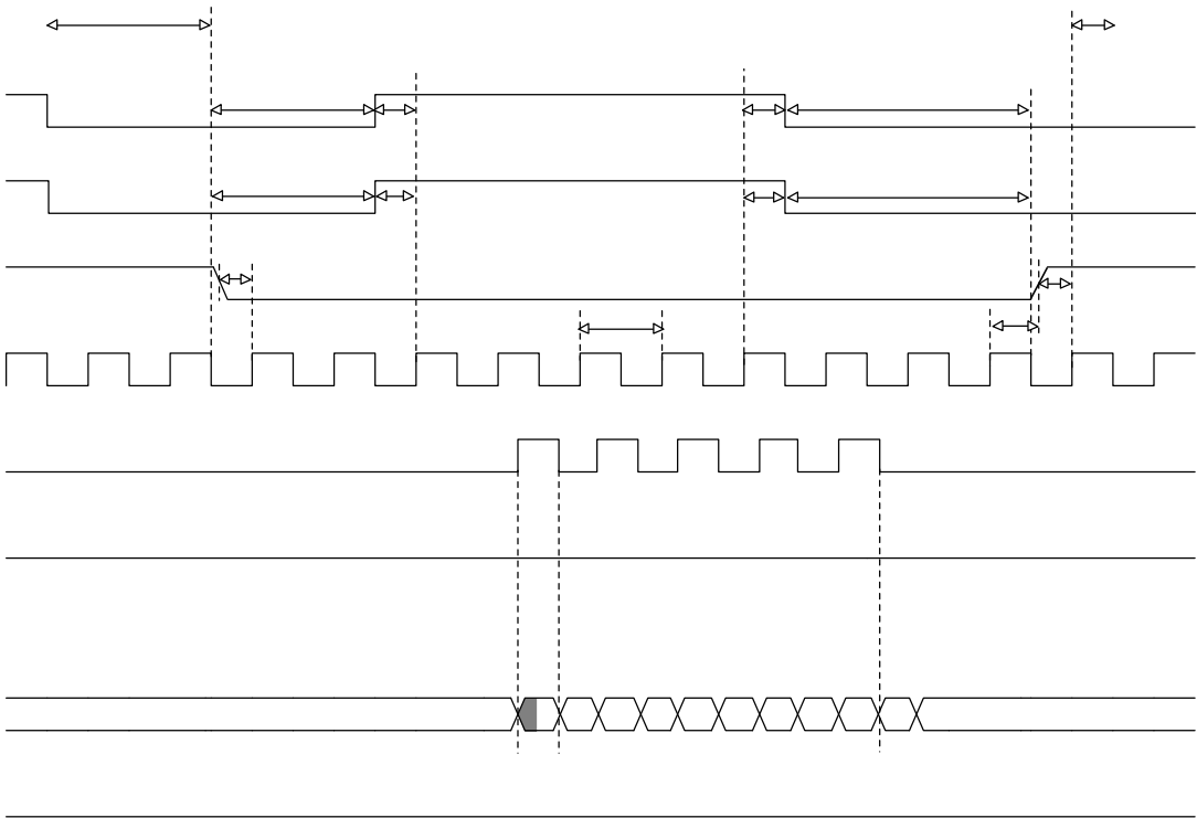
Figure 32. Source Synchronous Mode Data Read Timing Diagram
