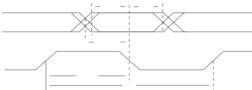
Figure 71. Data to Clock Timing Definitions
