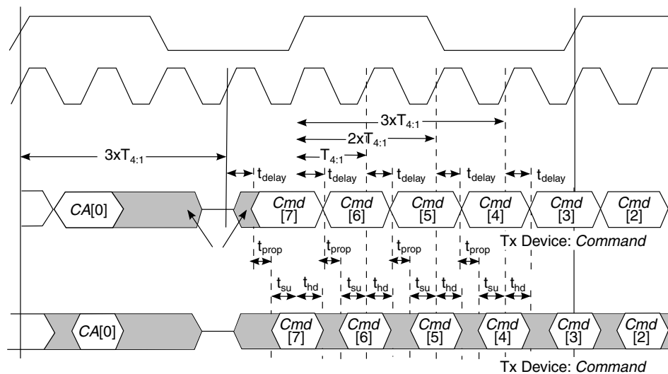
Figure 83. MLB 6-Pin Delay, Setup, and Hold Times
