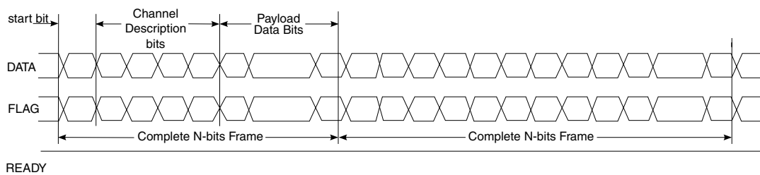
Figure 80. Frame Transmission Mode Transfer of Two Frames (Pipelined Data Flow)
