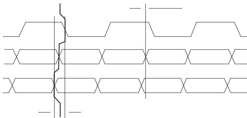
Figure 57. Inter-Pair Skew Definition
