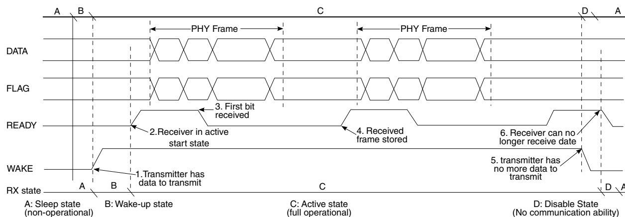
Figure 77. Synchronized Data Flow Transmission with WAKE
