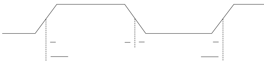
Figure 70. DDR Clock Definition
