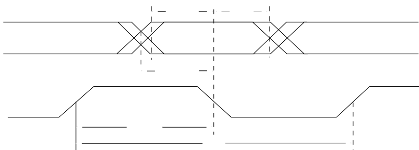
Figure 68. Data to Clock Timing Definitions
