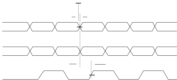
Figure 56. RGMII transmit signal timing diagram original
