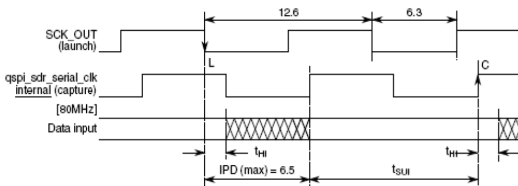
Figure 71. QuadSPI input timing (SDR mode)
