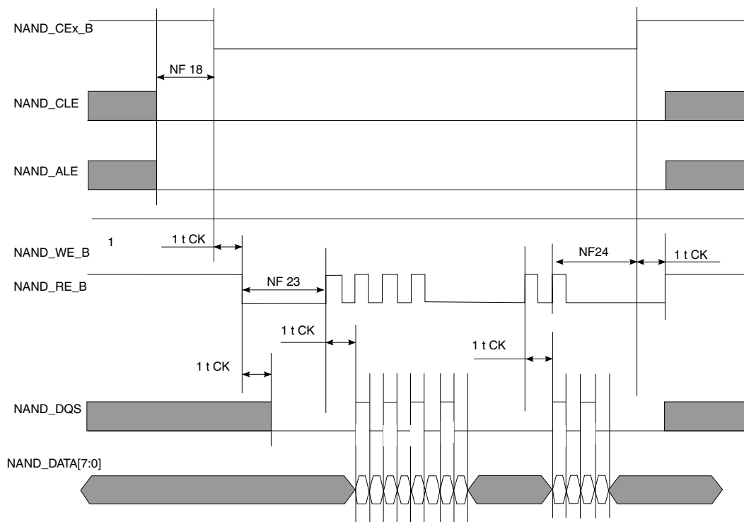
Figure 43. Toggle mode data read timing
