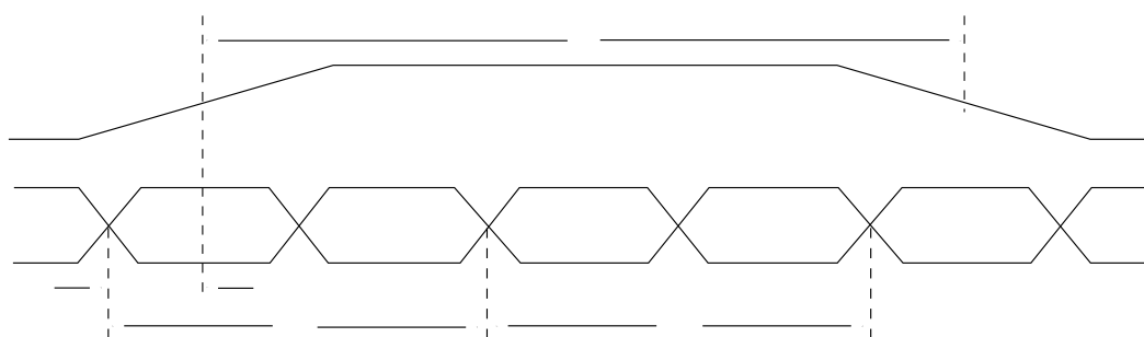
Figure 69. Reverse High-Speed Data Transmission Timing at Slave Side
