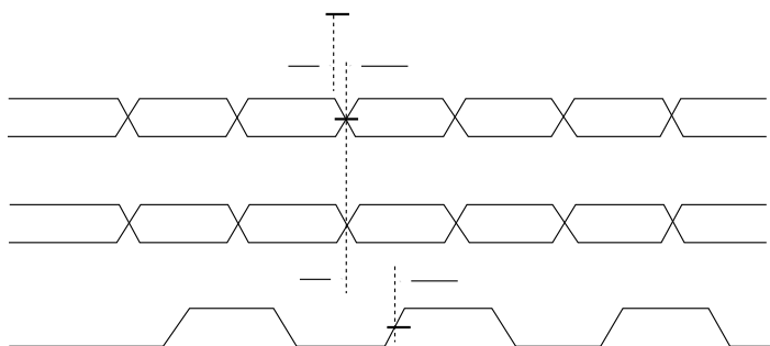
Figure 57. RGMII receive signal timing diagram original
