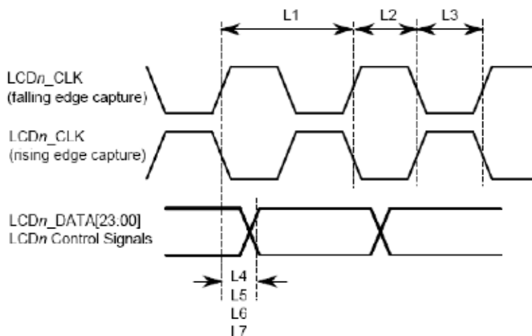
Figure 60. LCD timing
