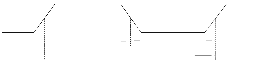
Figure 67. DDR Clock Definition
