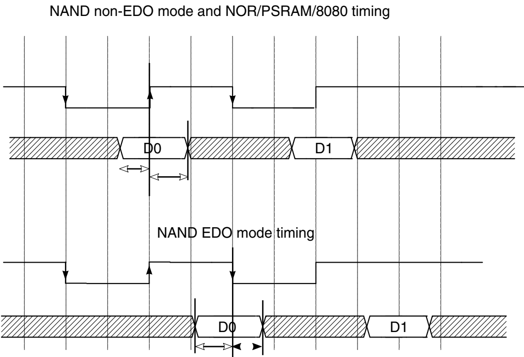
Figure 17. SEMC input timing in ASYNC mode
