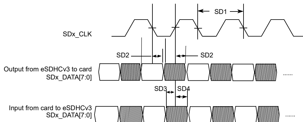
Figure 40. eMMC4.4/4.41 timing
