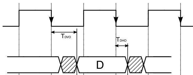
Figure 16. SEMC output timing in SYNC mode
