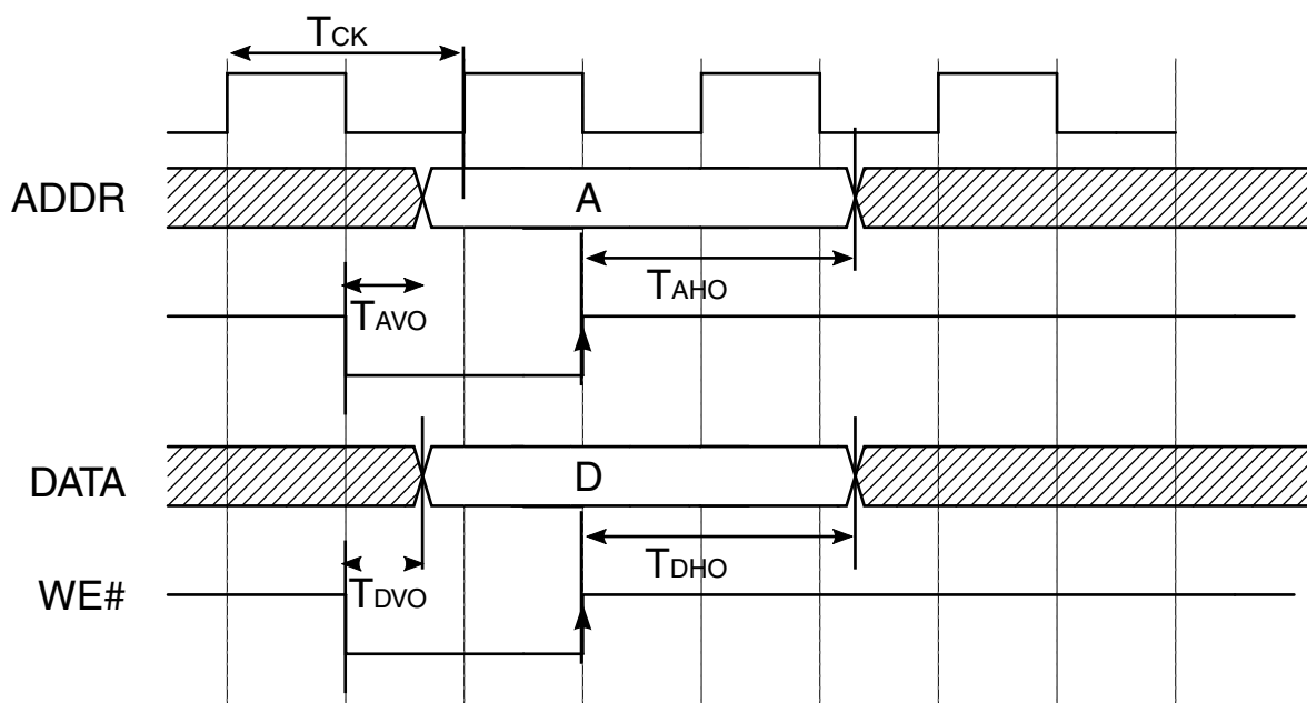
Figure 15. SEMC output timing in ASYNC mode
