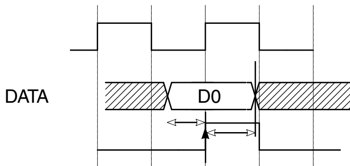
Figure 18. SEMC input timing in SYNC mode
