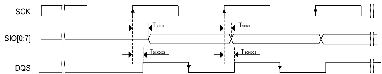
Figure 22. FlexSPI input timing in SDR mode where FlexSPI_MCR0[RXCLKSRC] = 0X3 (case A1)
