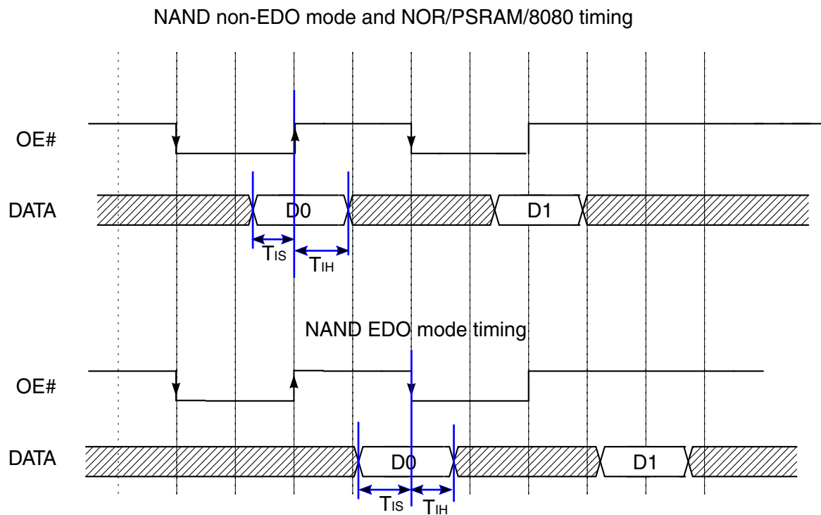
Figure 19. SEMC input timing in ASYNC mode
