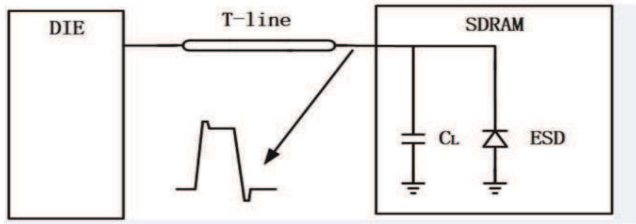
Figure 9. MCU-SDRAM circuit with overshoot/undershoot
