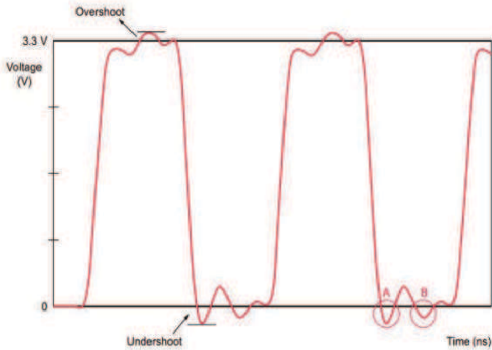
Figure 10. Overshoot and undershoot
