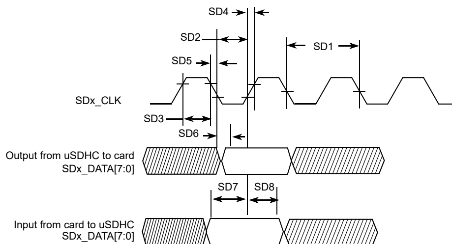
Figure 41. SD/eMMC4.3 timing
