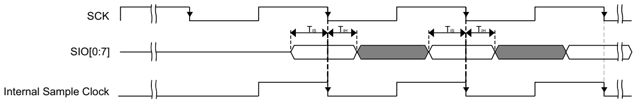
Figure 21. FlexSPI input timing in SDR mode where FlexSPI_MCR0[RXCLKSRC] = 0X0, 0X1
