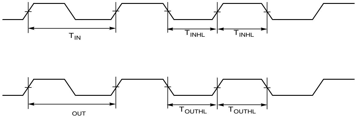
Figure 54. Quad timer timing
