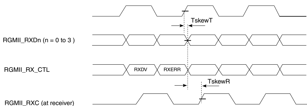
Figure 52. RGMII receive signal timing diagram
