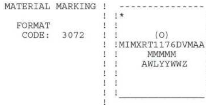
Figure 2. MAPBGA289 14 x 14 mm package marking format
