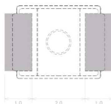
Figure 1. IN-P32ZTHIR Solder Pattern
