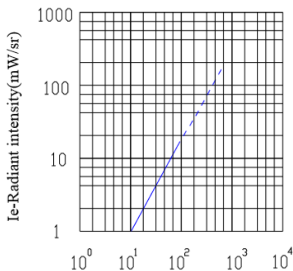
Relative Intensity & Forward Current
