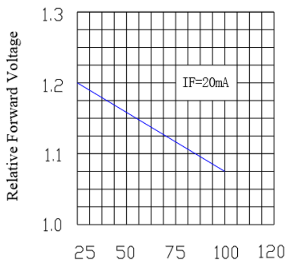
Forward Voltage & Ambient Temperature( ^{\circ}\text{C} )
