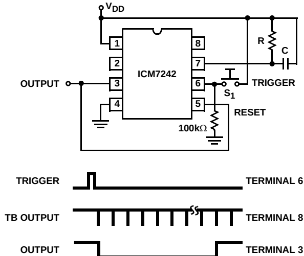
FIGURE 4. MONOSTABLE OPERATION
