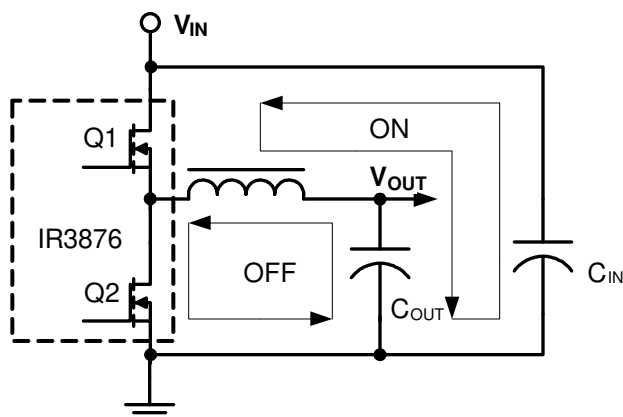
Figure 23. Current Path of Power Stage
