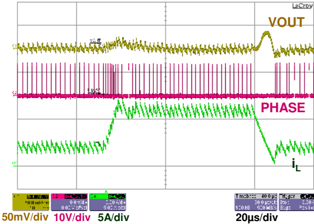
Figure 15: Load Transient 4-12A
