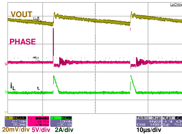
Figure 10: DCM ( I_{OUT} = 0.1A )
