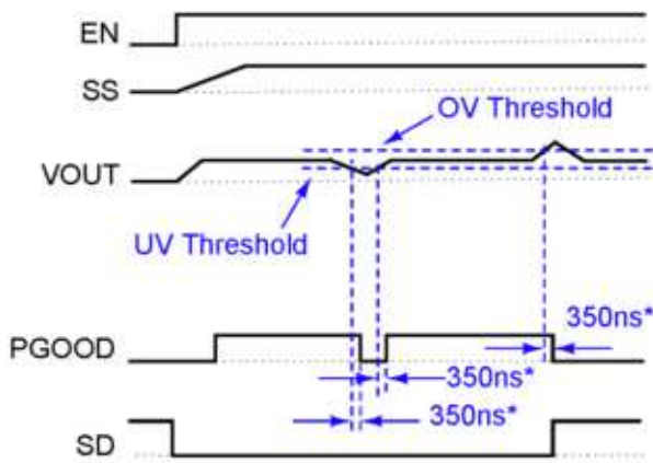
Figure 18(a). Under/Over Voltage Monitor
