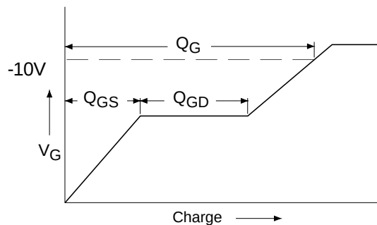
Fig 12a. Basic Gate Charge Waveform
