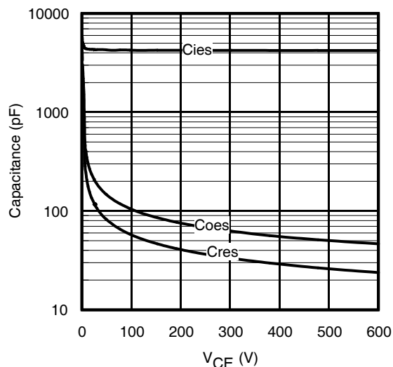
Fig. 24 - Typ. Capacitance vs. V_{CE}
