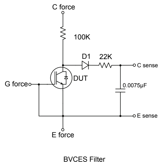
Fig.C.T.6 - BVCEs Filter Circuit
