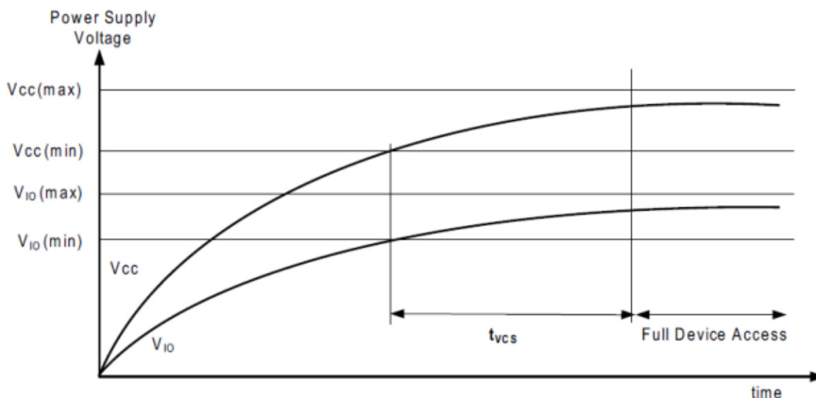
Figure 24. Power-Up
