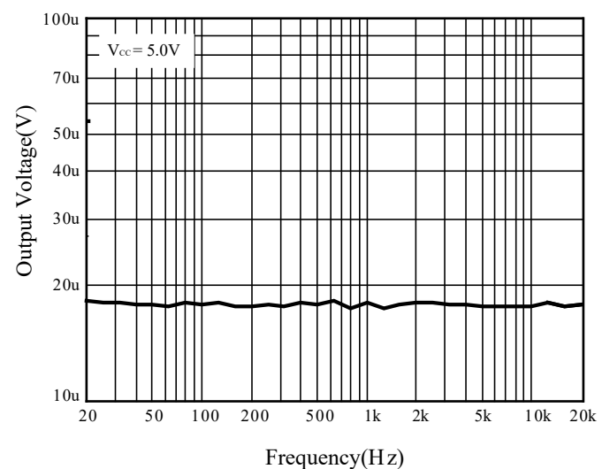
Figure 7 Noise Floor
