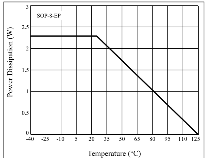
Figure 34 Dissipation Curve
