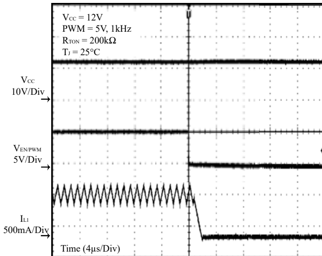
Figure 22 PWM Off
