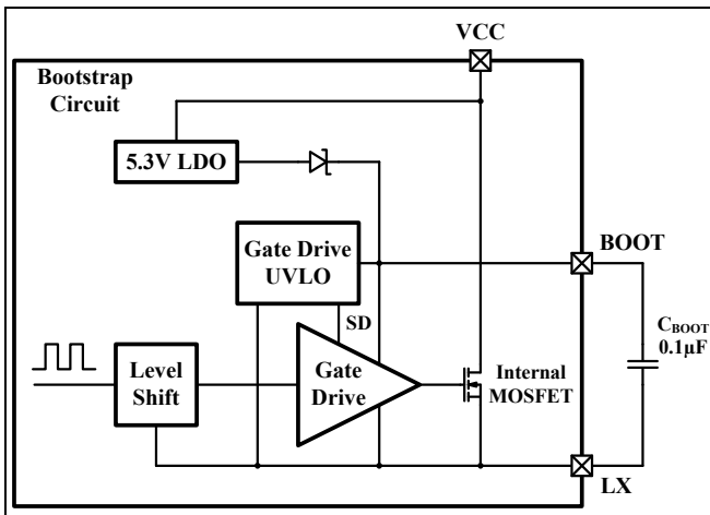
Figure 26 Bootstrap Circuit
