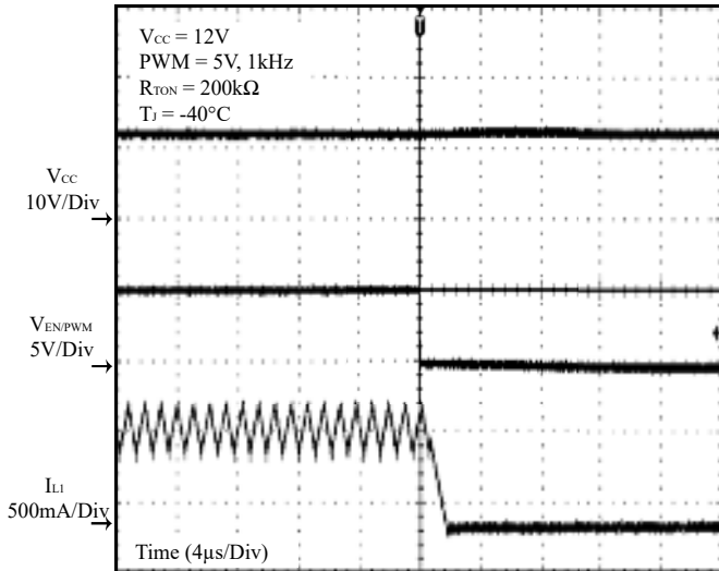
Figure 20 PWM Off
