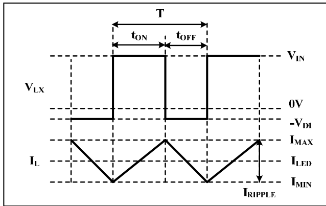
Figure 30 Operating Waveform
